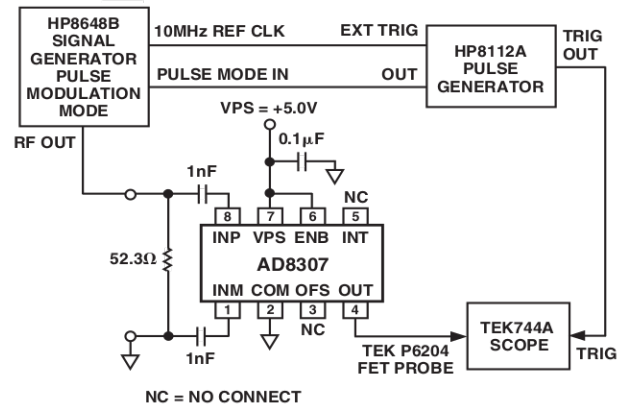
TPC 18. Test Setup for V_{OUT} Pulse Response
