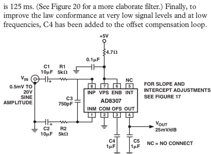
Figure 24. Connections for Low Frequency Operation
