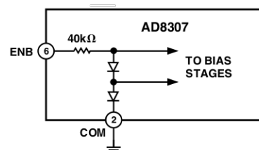
Figure 8. Enable Interface
