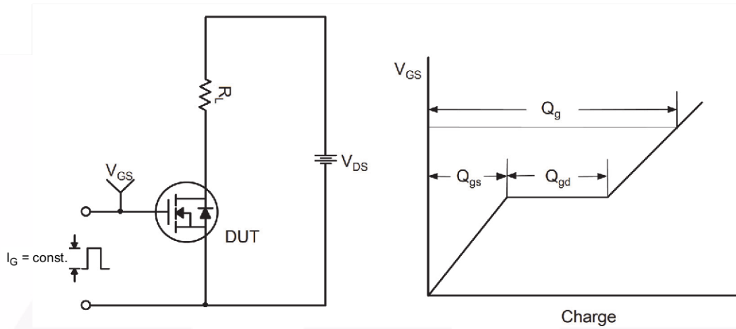
Figure 14. Gate Charge Test Circuit & Waveform
