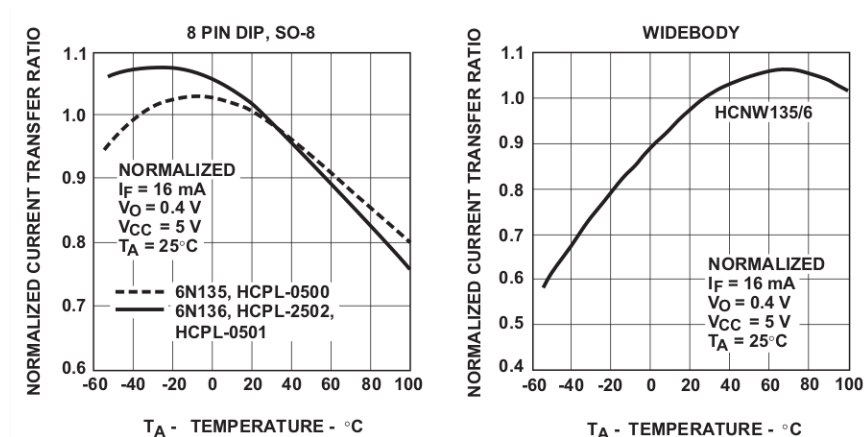
Figure 5: Propagation Delay vs. Temperature
