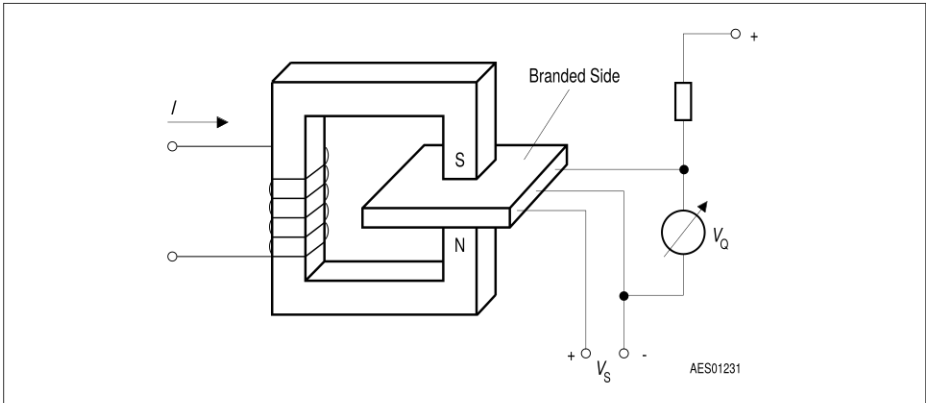
Figure 5 Sensor/Magnetic-Field Configuration
