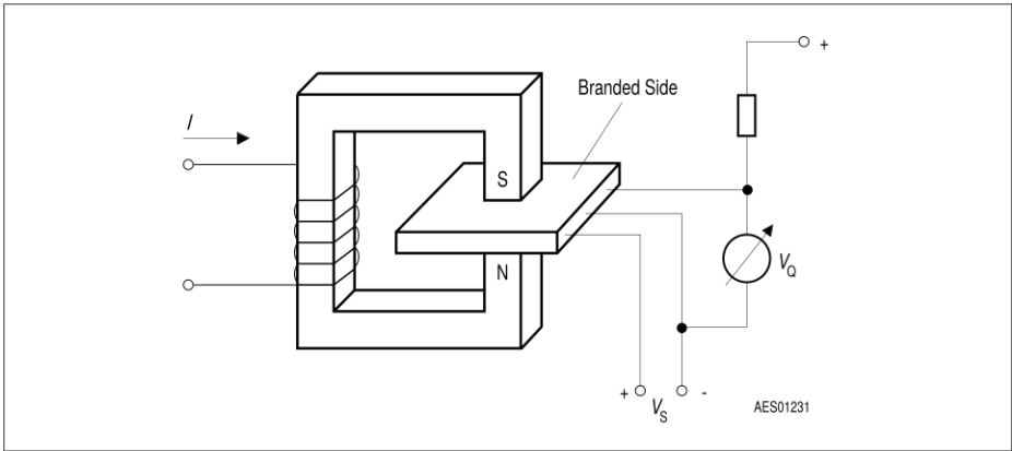
Figure 3 Sensor/Magnetic-Field Configuration
