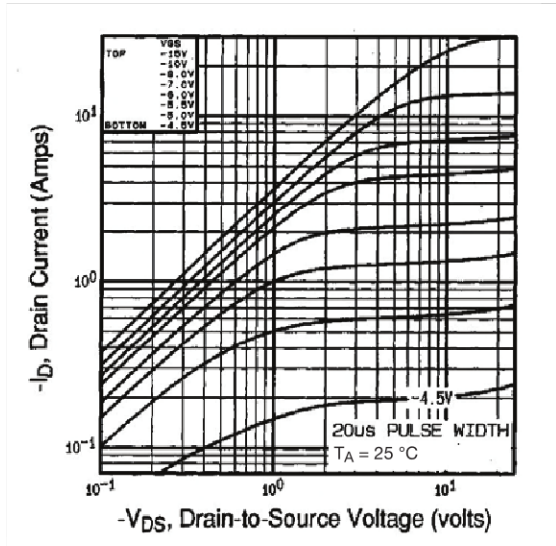
Fig. 1 - Typical Output Characteristics, T_A = 25\text{ °C}
