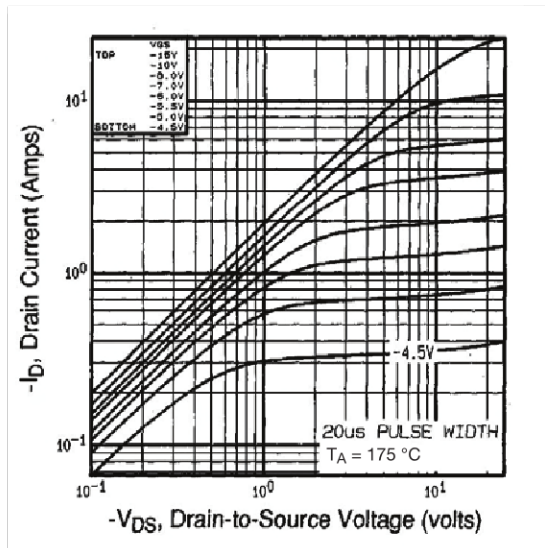
Fig. 2 - Typical Output Characteristics, T_A = 175\text{ °C}
