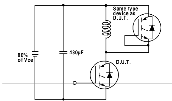
Fig. 18a - Test Circuit for Measurement of I_{LM} , E_{on} , E_{off}(\text{diode}) , t_{rr} , Q_{rr} , I_{rr} , t_{d(on)} , t_r , t_{d(off)} , t_f
