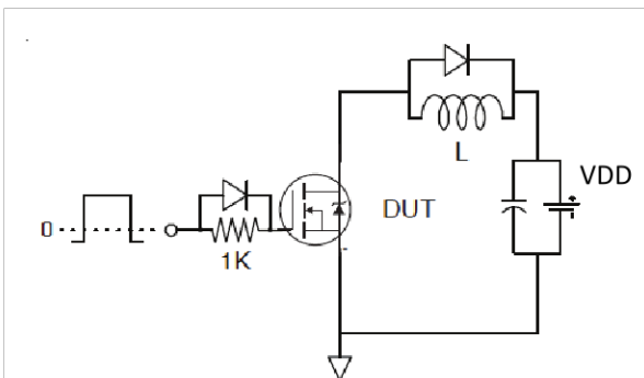
Fig 25a. Gate Charge Test Circuit
