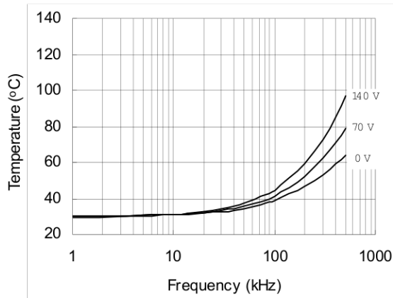
Figure 39. IRS21084S vs. Frequency (IRFBC40), R_{gate}=15 \Omega , V_{cc}=15 V
