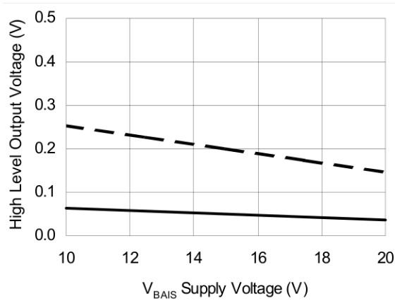
Figure 11B. High Level Output Voltage vs. Supply Voltage
