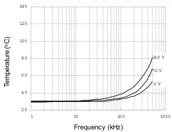
Figure 38. IRS21084S vs. Frequency (IRFBC30), R_{gate}=22 \Omega , V_{CC}=15 V
