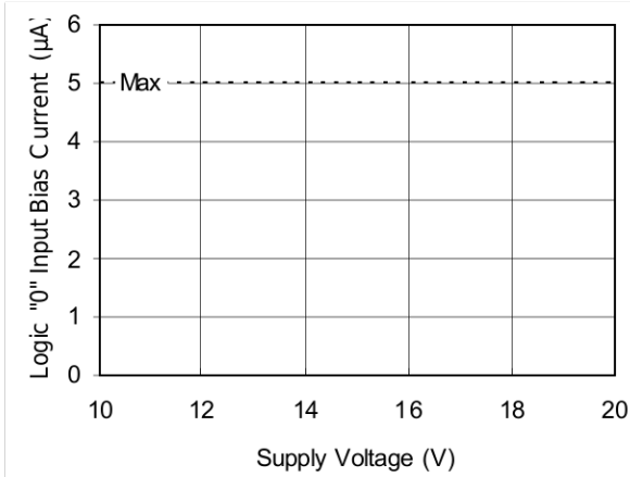
Figure 17B. Logic "0" Input Bias Current vs. Voltage
