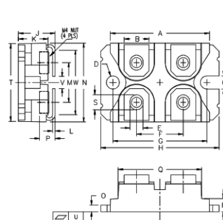
miniBLOC SOT-227 B M4 screws (4x) supplied
