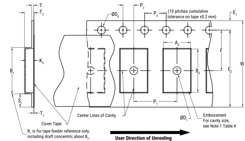
Figure 1 – Embossed (Plastic) Carrier Tape Dimensions
