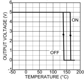
Shutdown Hysteresis vs. Temperature
