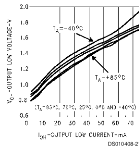
Driver V_{OL} vs I_{OL} vs Temperature
