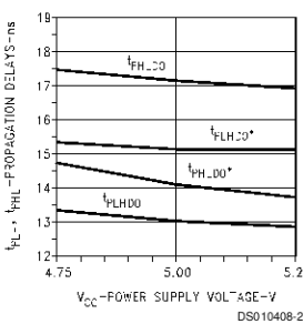
Driver Single-Ended Propagation Delay vs V_{CC}
