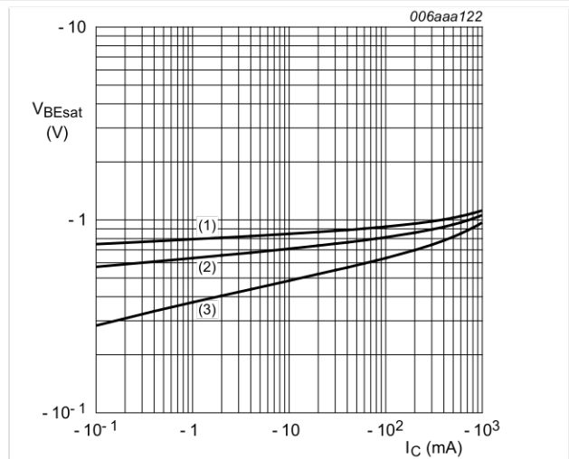
I_C/I_B = 10 (1) T_{amb} = -55\text{ °C} (2) T_{amb} = 25\text{ °C} (3) T_{amb} = 150\text{ °C}
