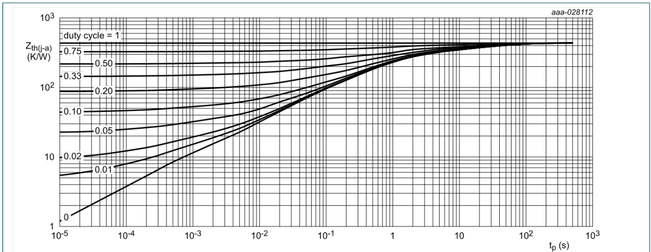
FR4 PCB, single-sided, tin-plated and standard footprint
