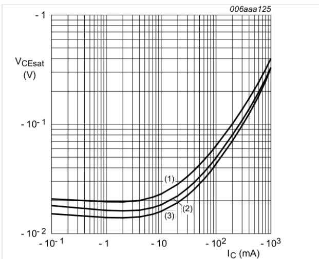
I_C/I_B = 10 (1) T_{amb} = 150\text{ °C} (2) T_{amb} = 25\text{ °C} (3) T_{amb} = -55\text{ °C}
