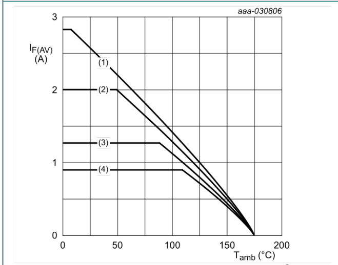
FR4 PCB, mounting pad for cathode 1\text{ cm}^2 T_j = 175\text{ }^\circ\text{C} (1) \delta = 1 ; DC (2) \delta = 0.5 ; f = 20\text{ kHz} (3) \delta = 0.2 ; f = 20\text{ kHz} (4) \delta = 0.1 ; f = 20\text{ kHz}
