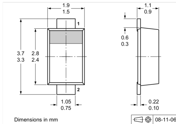
Fig. 18. Package outline CFP3 (SOD123W)
