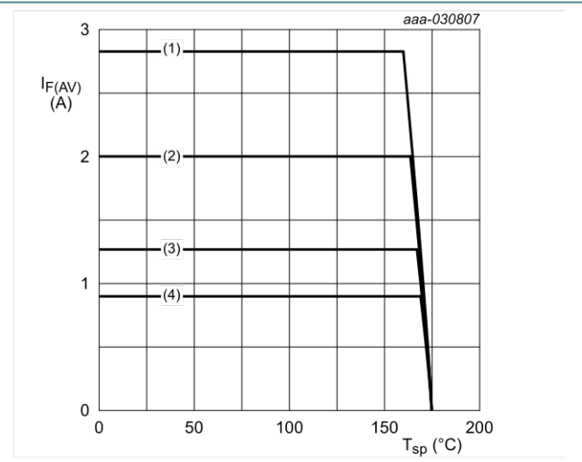
T_j = 175\text{ }^\circ\text{C} (1) \delta = 1 ; DC (2) \delta = 0.5 ; f = 20\text{ kHz} (3) \delta = 0.2 ; f = 20\text{ kHz} (4) \delta = 0.1 ; f = 20\text{ kHz}
