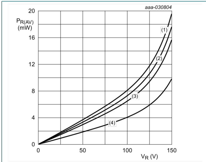
T_j = 175\text{ }^\circ\text{C} (1) \delta = 1 ; DC (2) \delta = 0.9 (3) \delta = 0.8 (4) \delta = 0.5
