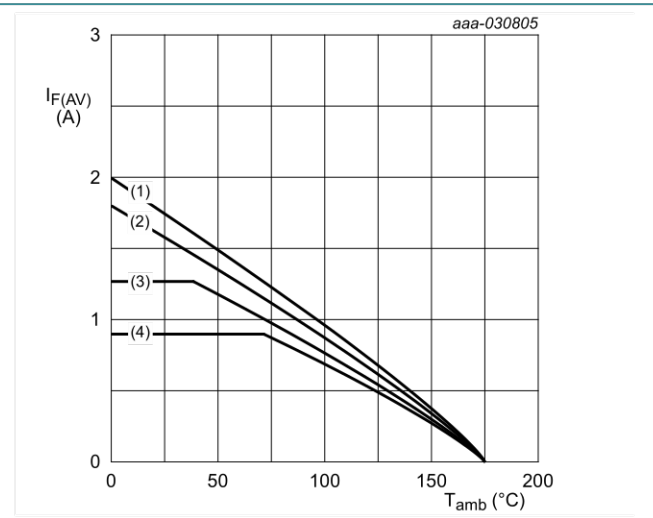
FR4 PCB, standard footprint T_j = 175\text{ }^\circ\text{C} (1) \delta = 1 ; DC (2) \delta = 0.5 ; f = 20\text{ kHz} (3) \delta = 0.2 ; f = 20\text{ kHz} (4) \delta = 0.1 ; f = 20\text{ kHz}
