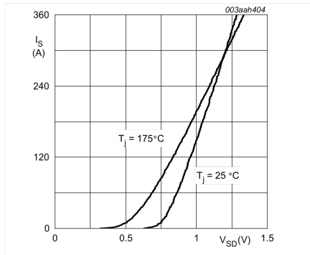
Fig. 16. Source (diode forward) current as a function of source-drain (diode forward) voltage; typical values
