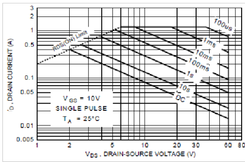
Figure 13. BS170 Maximum Safe Operating Area
