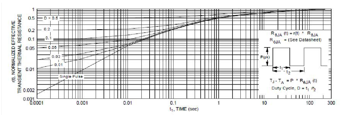
Figure 16. SOT-23, MMBF170 Transient Thermal Response Curve
