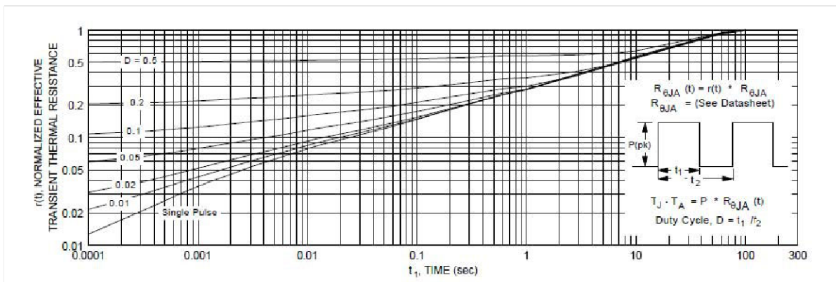
Figure 15. TO-92, BS170 Transient Thermal Response Curve
