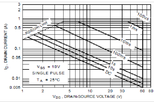
Figure 14. MMBF170 Maximum Safe Operating Area
