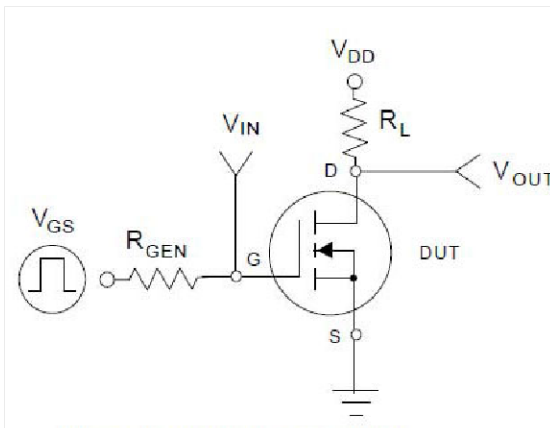
Figure 11. Switching Test Circuit
