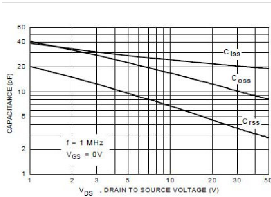
Figure 9. Capacitance Characteristics
