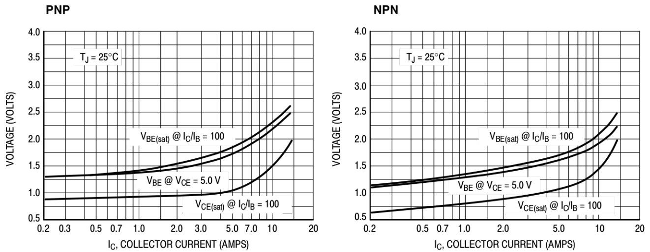
Figure 8. "On" Voltages
