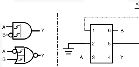
Figure 11. 2-Input AND with Inverted B Input
