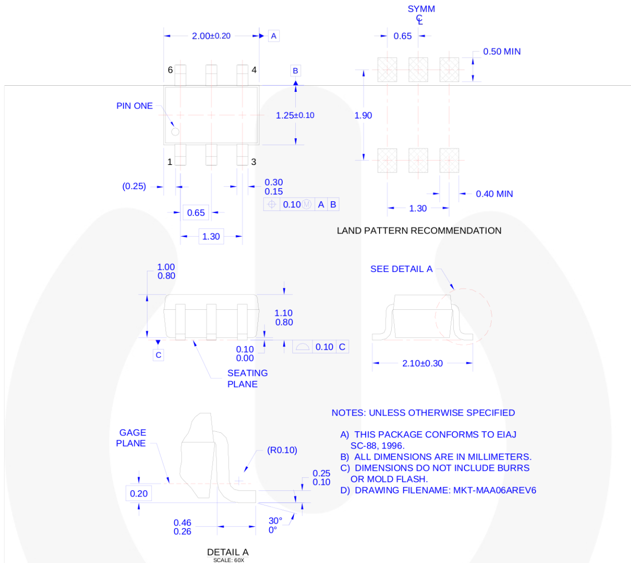
Figure 17. 6-Lead, SC70, EIAJ SC-88a, 1.25mm Wide
