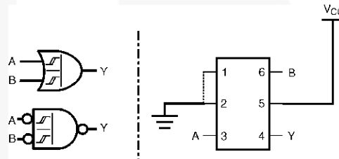
Figure 12. 2-Input OR Gate
