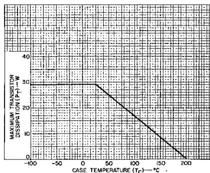
Fig. 2 - Dissipation derating curve for types 40310, 40312, 40316, and 40324.
