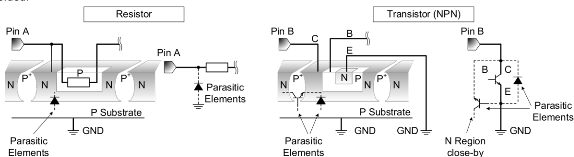
Figure 25. Example of IC Structure
