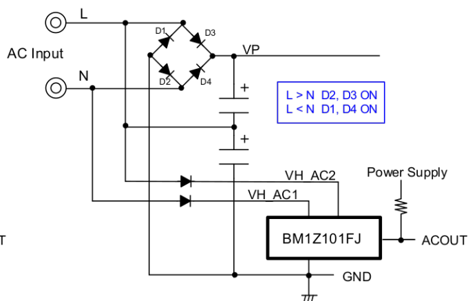
Figure 2. Double Voltage Rectification Circuit
