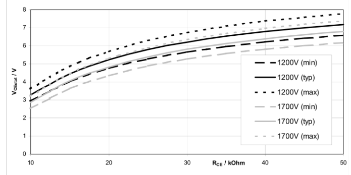
Fig. 4 V_{CEstat} in dependence of R_{CE} ( T_{amb} = 25^{\circ}C )
