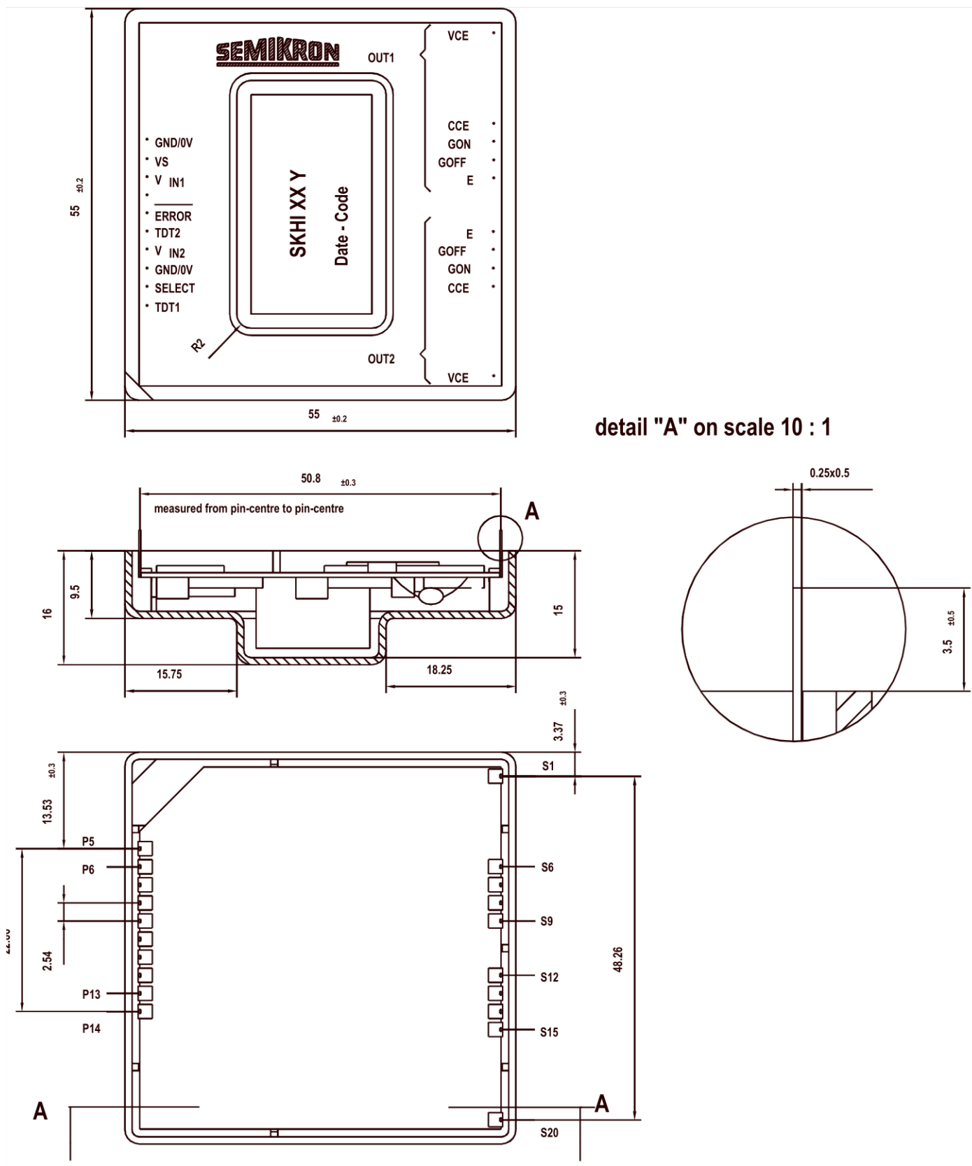
Fig. 2 Dimension drawing and PIN array (P5 and P6 are not existing for SKHI22A/21A)
