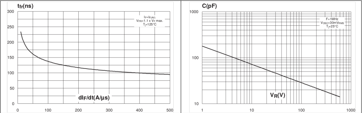
Figure 11. Forward recovery time versus dl_F/dt (90 % confidence) Figure 12. Junction capacitance versus reverse voltage applied (typical values)
