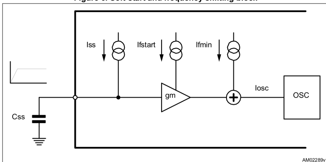
Figure 6. Soft-start and frequency shifting block
