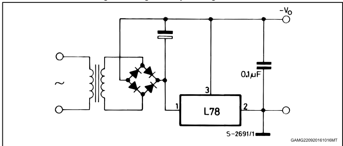
Figure 18: Switching regulator
