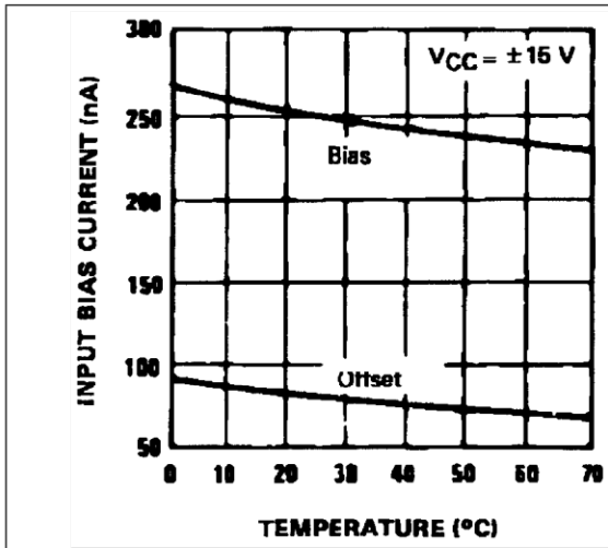
Figure 8. Input bias currents (LM319)
