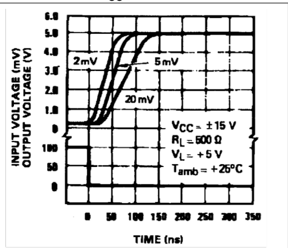
Figure 17. Response time on rising edge, V_{CC} = \pm 15\text{ V}
