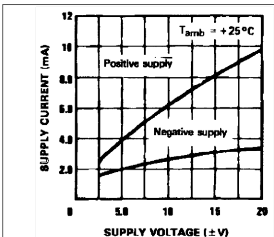
Figure 6. Supply current (LM119, LM219)
