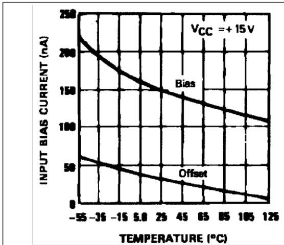
Figure 2. Input bias currents (LM119, LM219)
