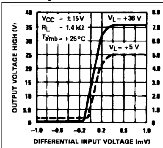
Figure 12. Transfer function
