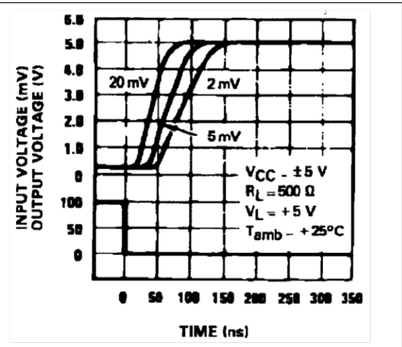
Figure 15. Response time on rising edge, V_{CC} = \pm 5\text{ V}
