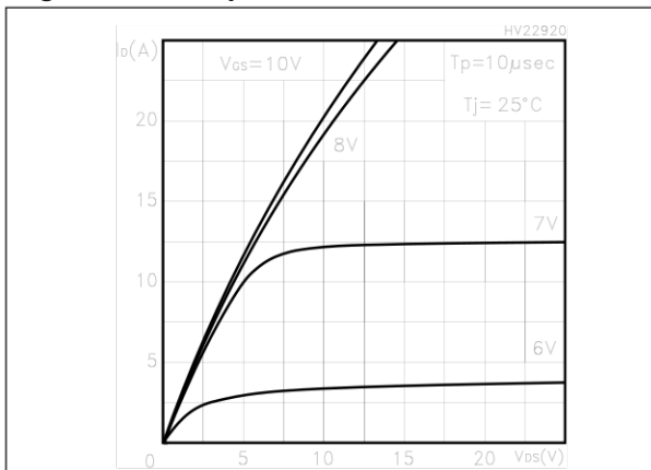
Figure 6. Output characteristics
