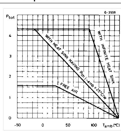
Figure 17. Maximum allowable power dissipation vs. ambient temperature
