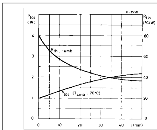
Figure 16. Maximum dissipated power and junction to ambient thermal resistance vs. side " \alpha "
