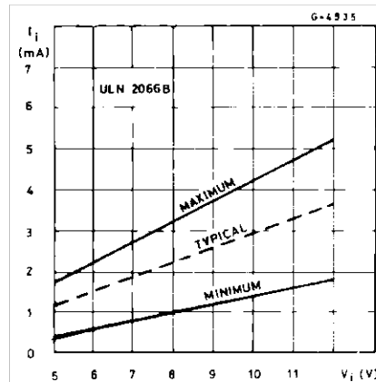
Figure 12. Input current as a function of input voltage
