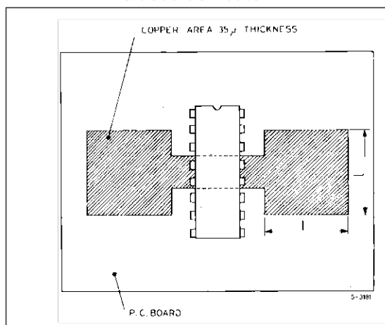
Figure 14. Example of P.C. board area which is used as heatsink
