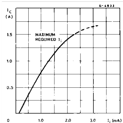
Figure 13. Collector current as a function of input current
