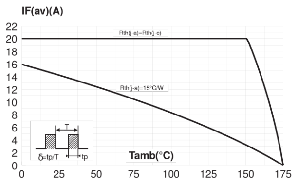
Fig. 2: Average current versus ambient temperature (per diode).
