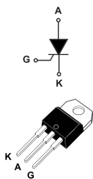
TO-220AB insulated
