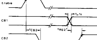
FIGURE 12 — CB2 DELAY TIME (Write Mode; CRB-5=1, CRB-3=CRB-4=0)
