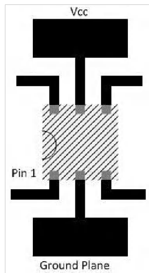
Figure 11-1. Recommended Layout Example
