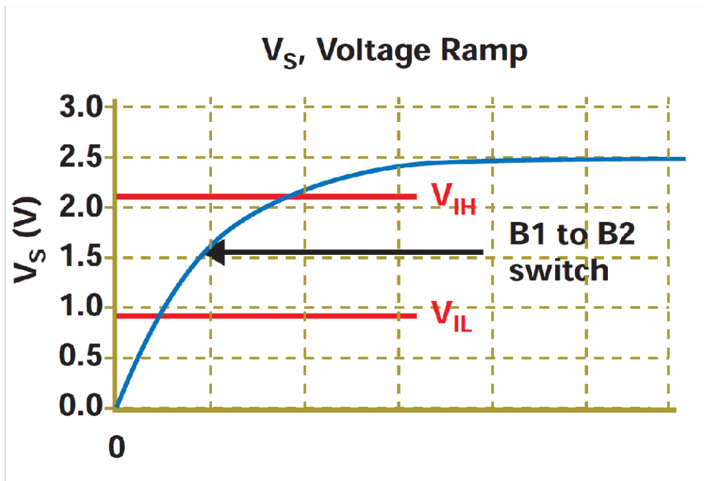
Figure 9-2. V S Voltage Ramp
