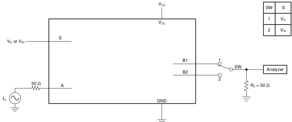
Figure 7-7. Feed Through
