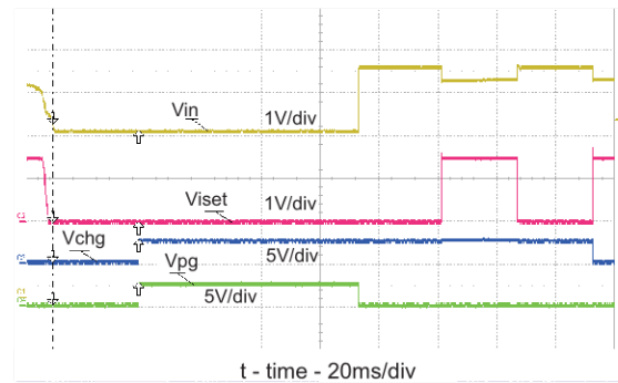
Figure 8-8. DPM – USB Current Limits – Vin Regulated to 4.4 V
