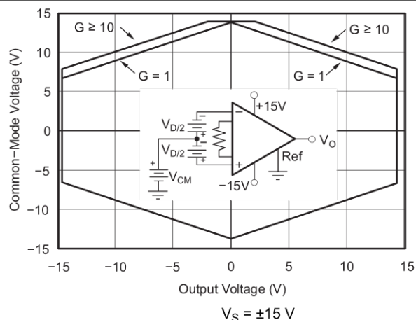
Figure 7-5. Input Common-Mode Range vs Output Voltage
