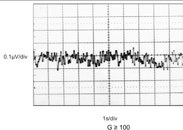
Figure 7-18. 0.1 to 10-Hz Input-Referred Voltage Noise
