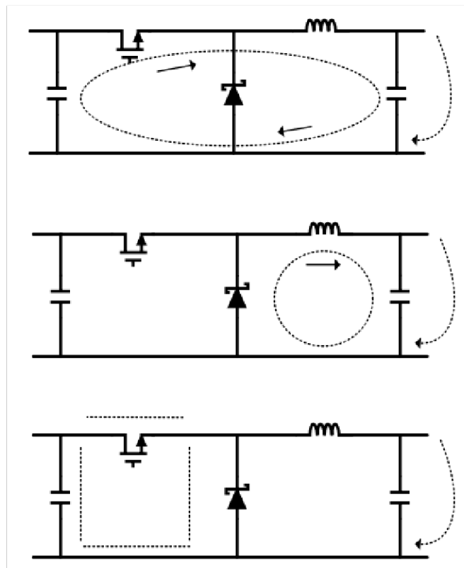
Figure 8-10. Current Flow in Buck Application
