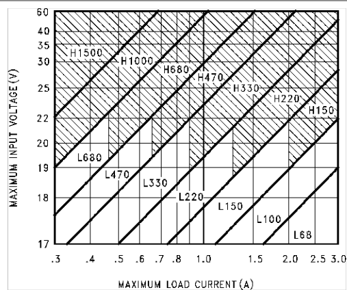
Figure 8-7. LM2576(HV)-15
