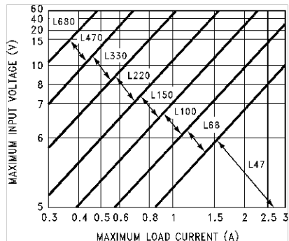
Figure 8-4. LM2576(HV)-3.3
