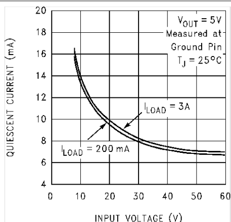
Figure 6-5. Quiescent Current
