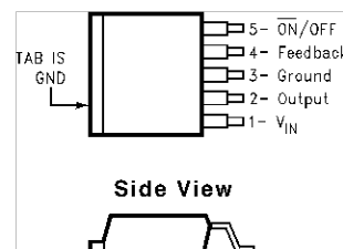
Figure 5-3. DDPAK/TO-263 (S) Package 5-Lead Surface-Mount Package Top View
