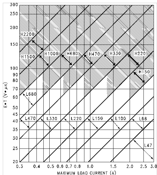
Figure 8-8. LM2576(HV)-ADJ
