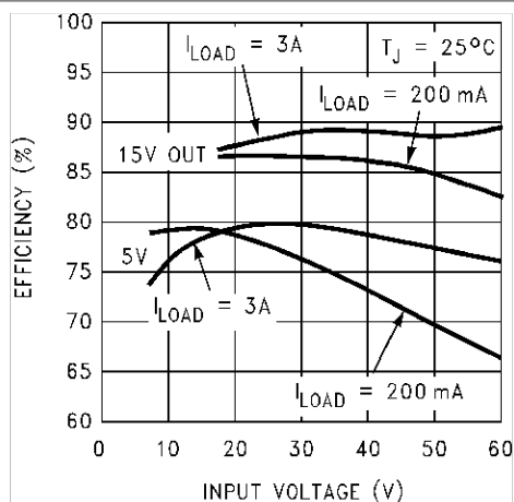
Figure 6-9. Efficiency
