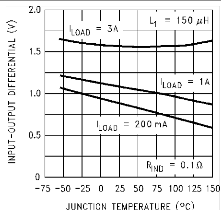
Figure 6-3. Dropout Voltage
