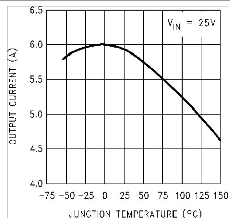
Figure 6-4. Current Limit
