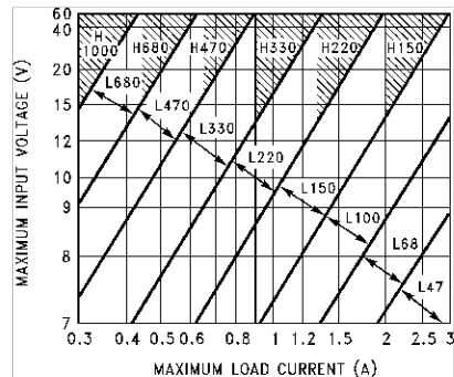
Figure 8-5. LM2576(HV)-5.0
