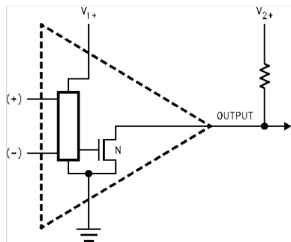
Figure 18. LMV7235 Open Drain Output
