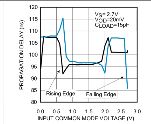
Figure 14. Propagation Delay vs. Common-Mode Voltage
