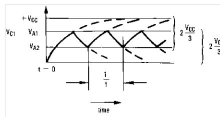
Figure 26. Square Wave Oscillator Timing Thresholds
