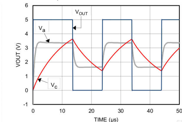
Figure 27. Square Wave Oscillator Output Waveform
