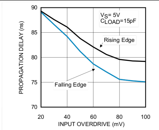
Figure 13. Propagation Delay vs. Input Overdrive
