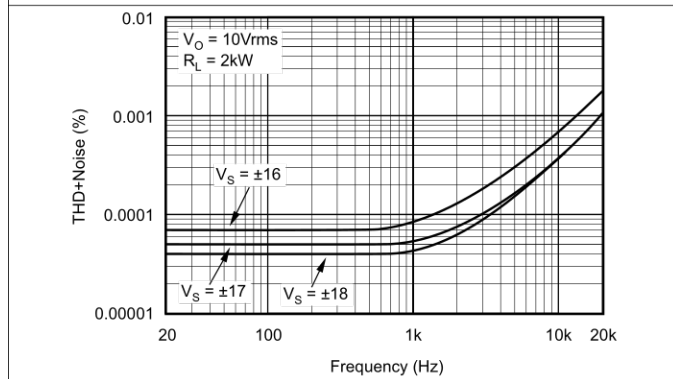
Figure 1. Total Harmonic Distortion + Noise vs Frequency
