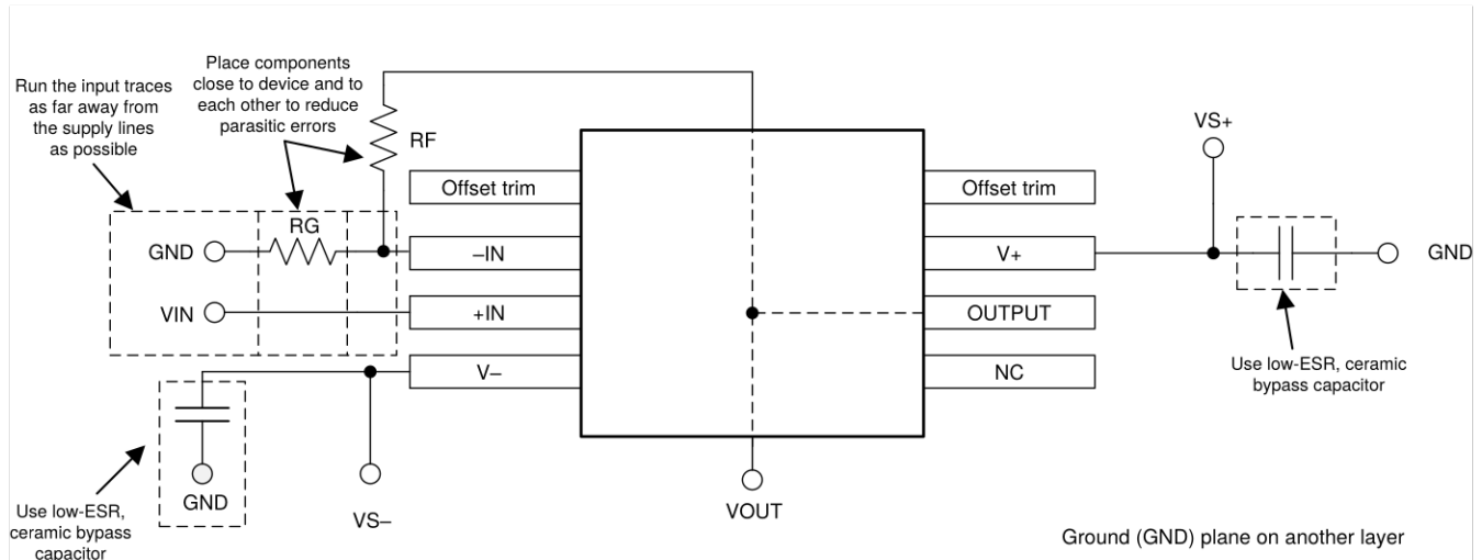
Figure 32. OPA134 Layout Example for the Noninverting Configuration
