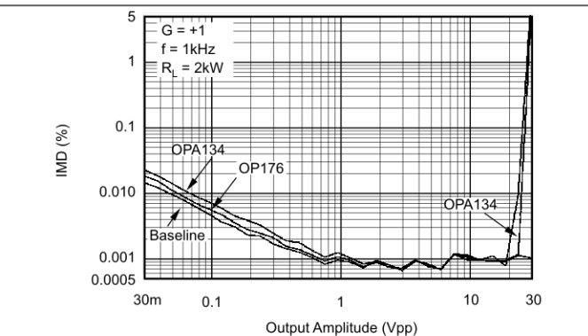
Figure 2. SMPTE Intermodulation Distortion vs Output Amplitude
