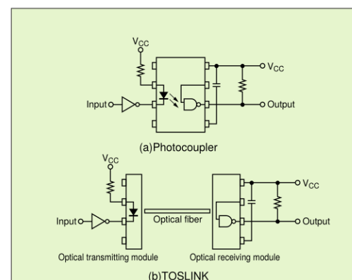
Comparison of TOSLINK and photocoupler
