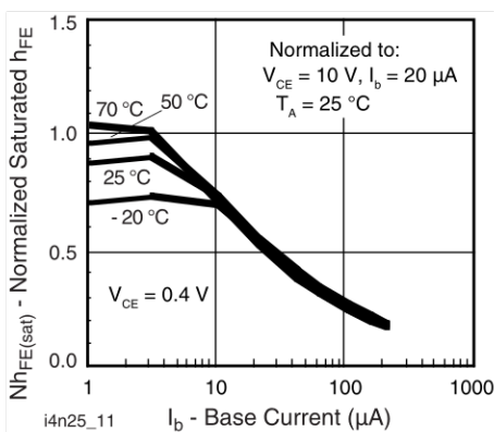
Fig. 11 - Normalized h_{FE} vs. Base Current and Temperature
