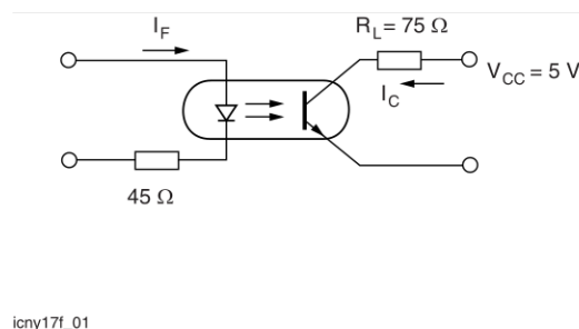
Fig. 1 - Linear Operation (without Saturation)
