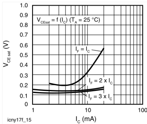
Fig. 15 - Saturation Voltage vs. Collector Current and Modulation Depth CNY17F-4
