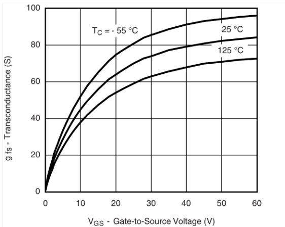
Transconductance
