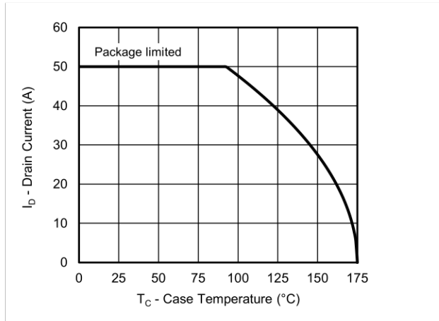
Max. Avalanche and Drain Current vs. Case Temperature
