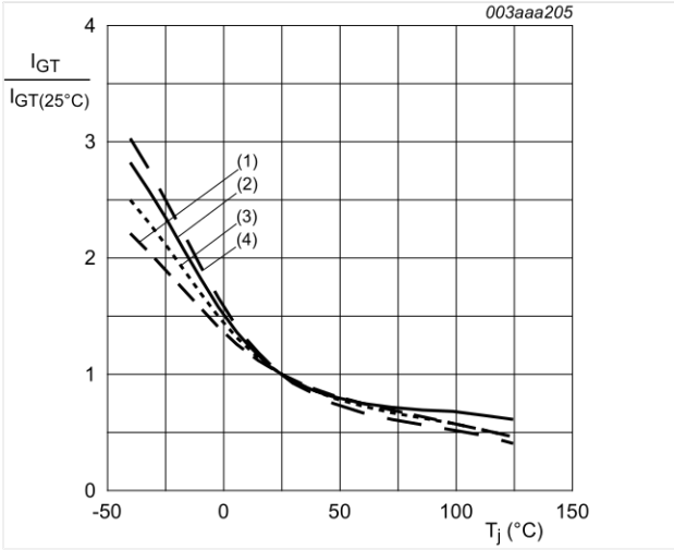
Fig. 9. Normalized gate trigger current as a function of junction temperature
