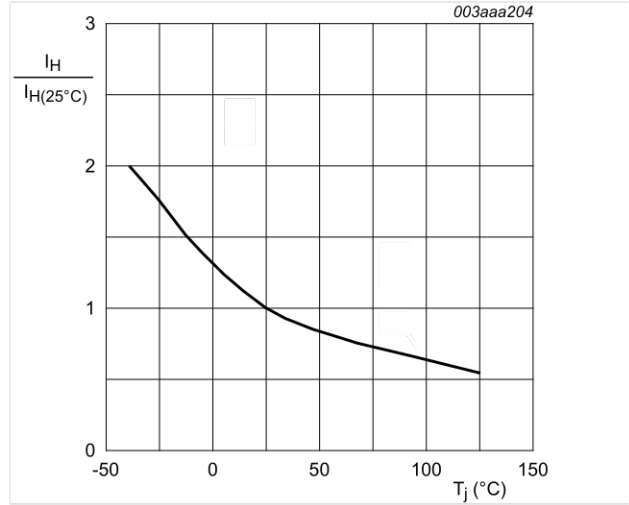
Fig. 10. Normalized holding current as a function of junction temperature
